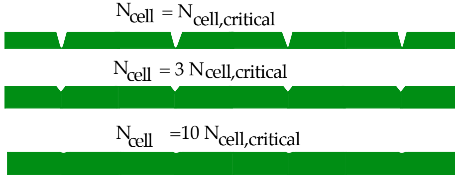
Fig. 3 Toy Models. Correlation functions g(\mathbf{r}_{12}) are shown for three values of N_{cell} . The cusp depth becomes deeper with decreasing N_{cell} . At N_{cell,critical} the values of g(\mathbf{r}_{12}) \rightarrow 0 at each \mathbf{r}_{12} = 0 modulo \mathbf{R}_{12j} .
