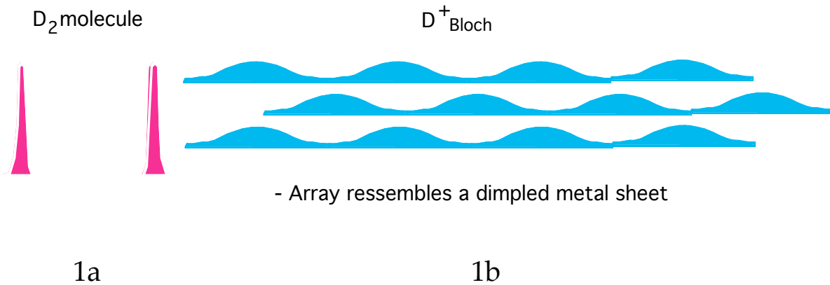
Fig. 1 Toy Models: Fig. 1a shows the charge distribution of two D^+ in separated potential wells within a molecule's electron cloud. The deuterons are mutually incoherent. The Leggett and Baym modeling (6) has incoherence of this type. Fig. 1b shows a single Bloch D^+ in an array of potential wells provided by a metal crystal. Neutralization is provided by the metal's mobile electrons. Localized charge maxima are coherently coupled so that the sum over N_{\text{cell}} unit cells is a single delocalized deuteron. Fig. 1b can also depict the center-of-mass charge distribution of two Bloch D^+ ions coherently coupled by coordinate exchange, and also of a quasiparticle pairing of Bloch deuterons in a many-body D^+ Bloch system. The array of charge maxima is used to illustrate both a D^+ charge distribution having 3-dimensional periodic symmetry inside a metal, and a D^+ charge distribution inside an interface layer resting on metal surface having 2-dimensional periodic symmetry.
