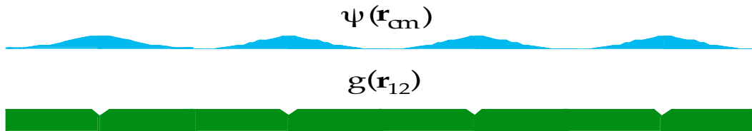
Fig. 2 Toy Model. Factor e|\psi(\mathbf{r}_{\text{cm}})|^2 measures the charge distribution of 2\text{-D}^+_{\text{Bloch}} in center-of-mass space \{\mathbf{r}_{\text{cm}}\} , which is also lattice space. The
